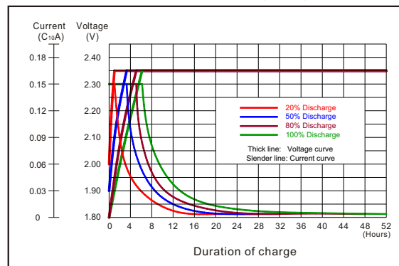
Charging Characteristics Curves (25°C)
