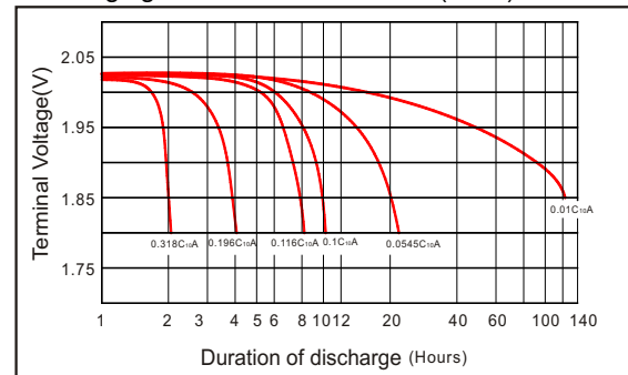
Discharging Characteristics Curves (25°C)
